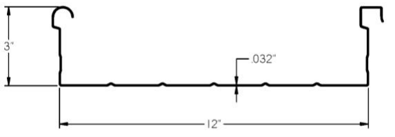
Roll Form Flat Pan
