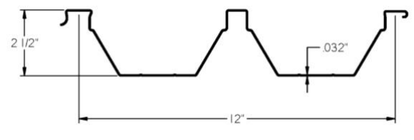
Roll Form W-Pan
