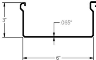
Extruded Flat Pan
