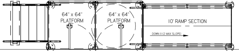
STEP AND RAMP WITH DOUBLE DOORS
