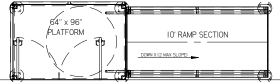
RAMP WITH DOUBLE DOORS
