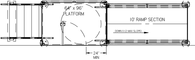
STEP AND RAMP WITH SINGLE DOOR
