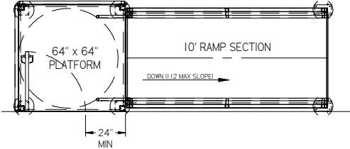
RAMP WITH SINGLE DOOR
